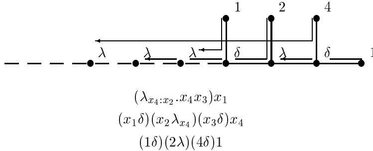
Figure 4: A tree with de Bruijn's indices
