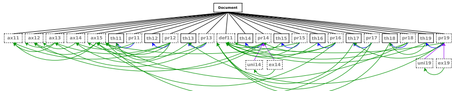
Figure 3: The DG of sections 1 and 2 of chapter 1 of Landau's book
