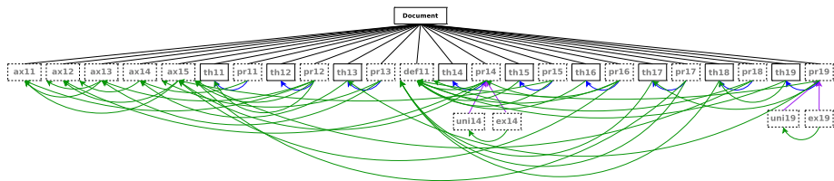
Figure 3: The DG of sections 1 and 2 of chapter 1 of Landau's book
