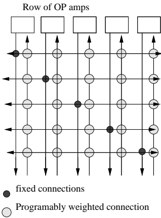
Figure 1: A fully interconnected array.
