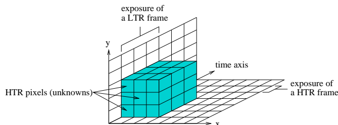
Figure 2: Image formation model in the discrete domain. Each LTR pixel (darker box) is a weighted average of several HTR pixels (smaller boxes).
