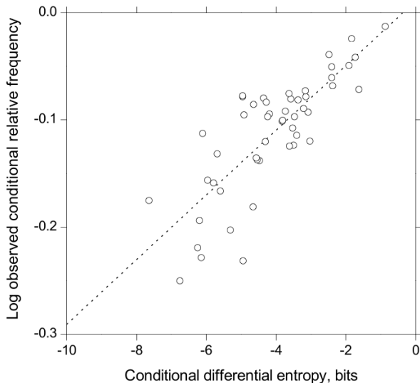
Figure 1. Predicting how often an indistinguishable pair of surfaces under sunlight (CCT 4000 K) becomes distinguishable under north skylight (CCT 25,000 K). The logarithm of the observed conditional relative frequency of metamerism is plotted against estimated conditional differential entropy. The dotted line is a linear regression.
