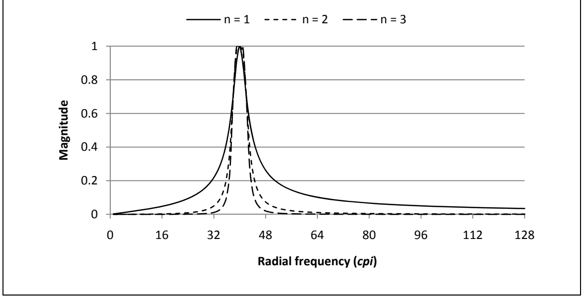
Figure 5-4: Effect of Butterworth order on distribution of radial frequency components
