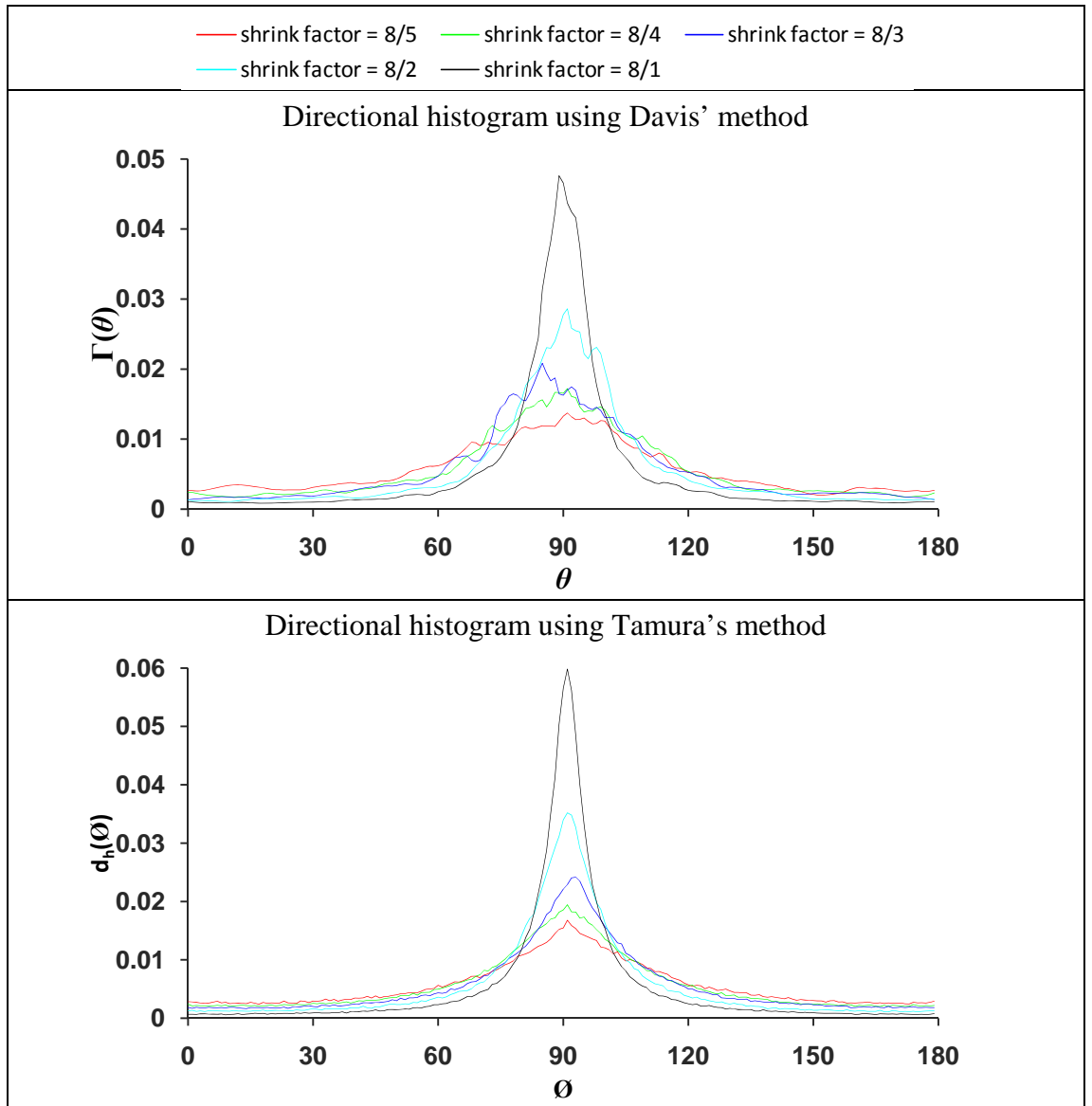
Figure 3-6: Directional histograms of the surfaces from set 1
