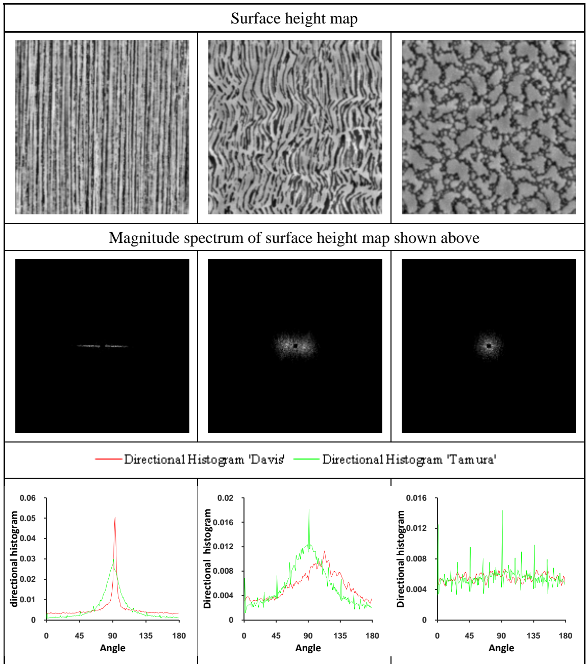
Figure 3-1: Effect of distribution of frequency components on the computational directionality.
