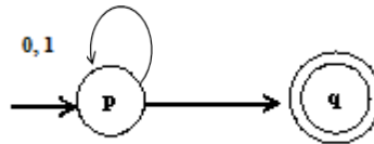
Figure 3: M1 a NonDeterministic Finite Automaton
