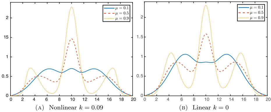
FIGURE 7. Solution of (2.1) at the end time T = 4 approximated with the scheme (6.1) with a = 1 , r = 0 and varying values of \mu \in (0, 1)
