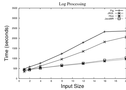
Fig. 7. Web Log Processing Scale Up - Uniform Distribution
