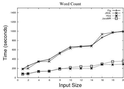
Fig. 6. Word Count Scale Up - Uniform Distribution
