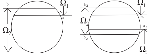
FIGURE 1. Latitudinal domain decomposition. Left: two domains; right: multiple domains.
