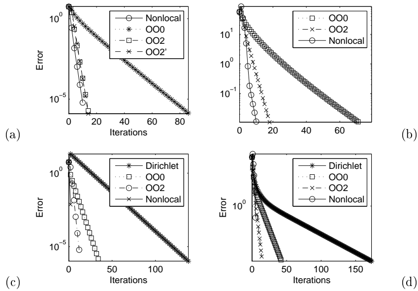
FIGURE 2. Numerical results, semispectral code. (a): convergence with two latitudinal subdomains and zero overlap. (b): convergence with six latitudinal subdomains and zero overlap. (c): convergence with two latitudinal subdomains and two grid lengths of overlap. (d): convergence with six latitudinal subdomains, the overlaps are each the length of one grid interval.
