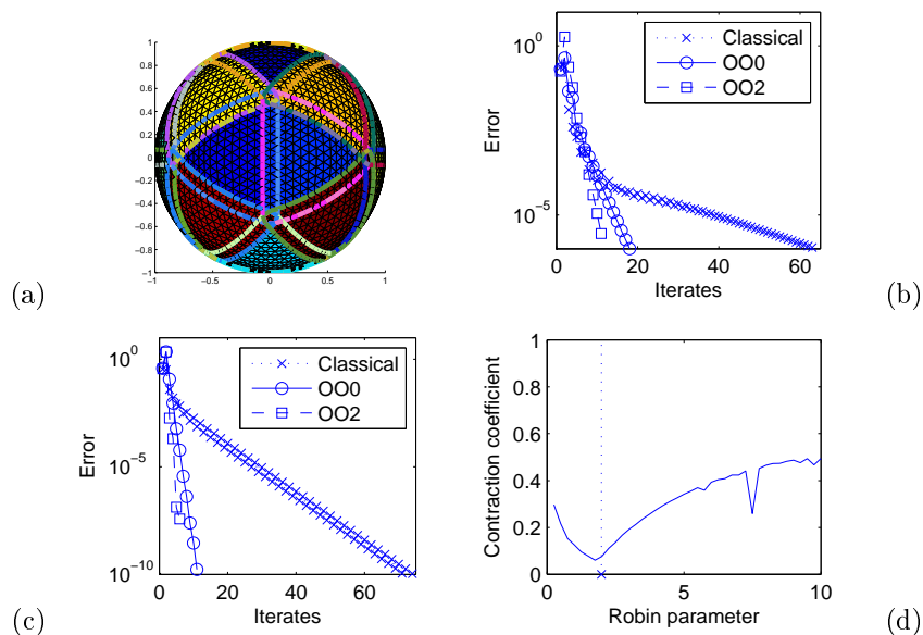
FIGURE 3. (a): An icosahedral grid with 20 subdomains. (b): Convergence of classical and optimized Schwarz methods for the grid of (a). (c): Convergence of classical and optimized Schwarz methods, for two nearly hemispherical overlapping subdomains, (d): The accuracy of the optimized Schwarz coefficient chosen in (c).
