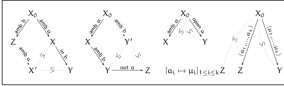
Figure 5: Definition 4.2 in diagram form
