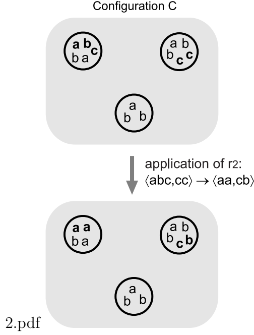
Fig. 2. Application of an instance of the synchronization rule r_2 to configuration C from Example 1.
